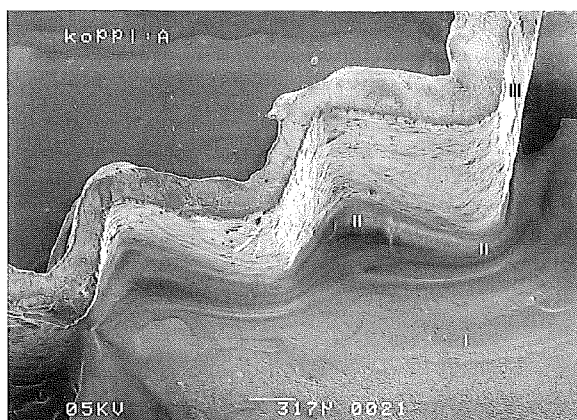
Figure 2. SEM photograph of head-plate A. Magnification 31.5 ×. I = gold sheet, II = soldering seam, and III = cell wall (photo GIA).
