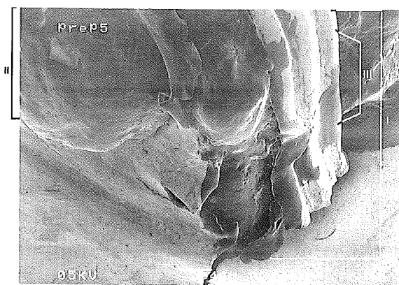
Figure 7. SEM photograph of the hinge. Magnification 13.4 ×. I = vertical section of silver- and copper alloy, II = detail of copper alloy pin, and III = ribbed gold edging covering the silver and copper alloy (photo GIA).
